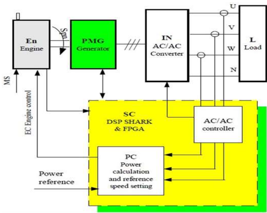
Figure 1. Block diagram of overall variable speed power generation system
