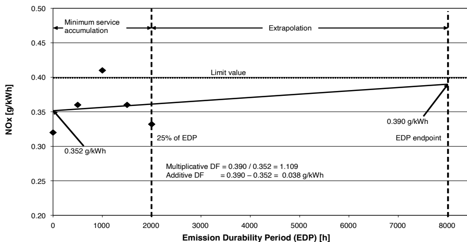
Figure A.8-1. Example of DF determination
