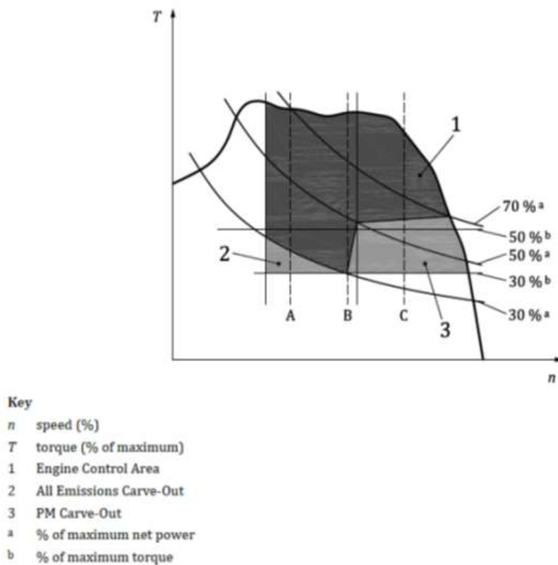
Figure 1 – Engine control area for Engines tested to cycles C1, C > 2400 rpm
