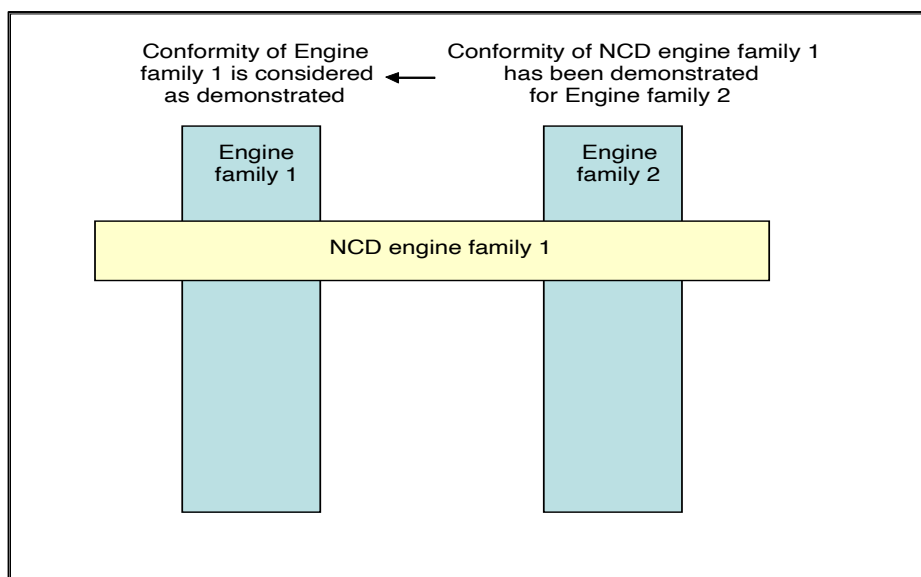
Figure A.8-3. Previously demonstrated conformity of an NCD engine family
